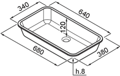
Technical Drawing
